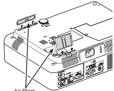
Air filters Pull up and remove.
